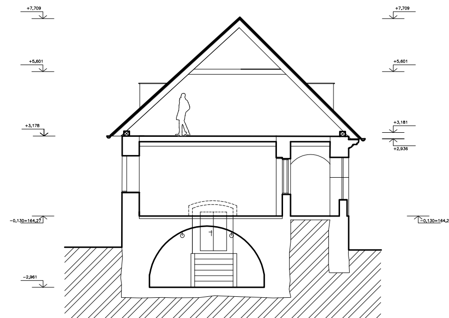
REZ AA M 1:100
