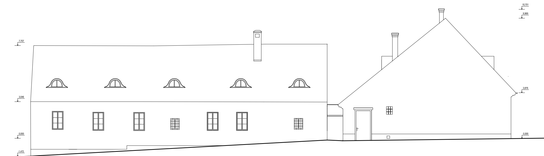
POHLAD SEVERNÝ
