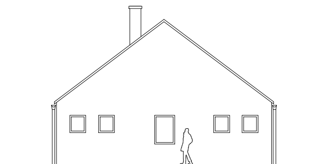
POHLAD SEVERNÝ
