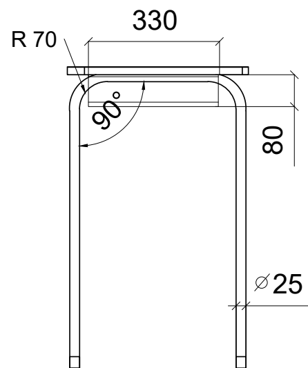
bokorys
