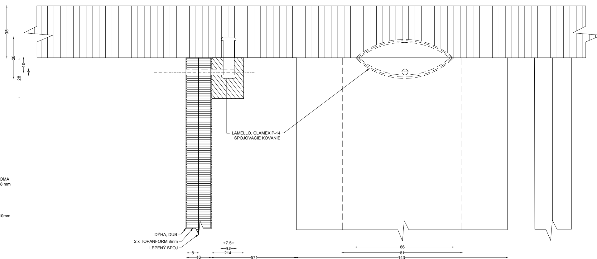
DETAIL A
