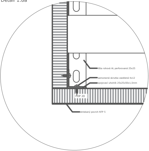
Detail 1.8a
