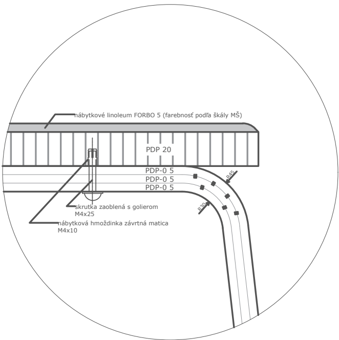
Detail 1.7a
